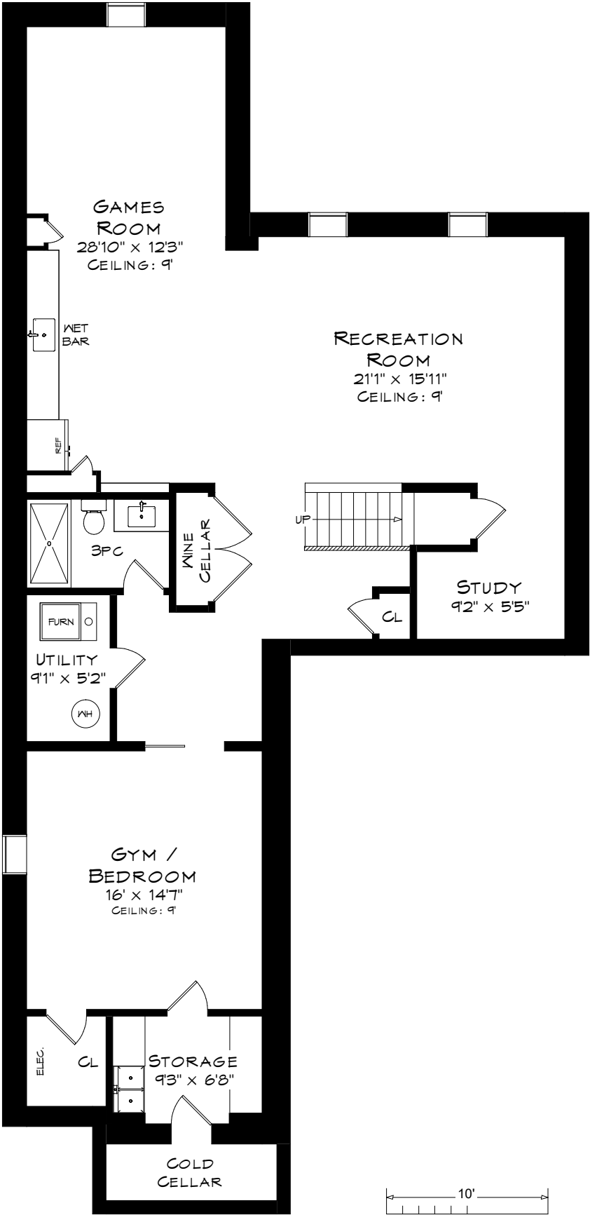
LOWER LEVEL 1,782 SQUARE FEET
